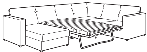
VIMLE corner sofa-bed, 5-seat with chaise longue. Total size: W349/249×D98/241×H83 cm. NA: W362/249×D98/241×H83 cm (W142½/98×D38⅝/94⅞×H32⅝"). Storage in the chaise longue.
