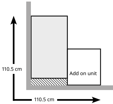
58 cm deep add-on unit for corner with one 100×58 cm frame.
